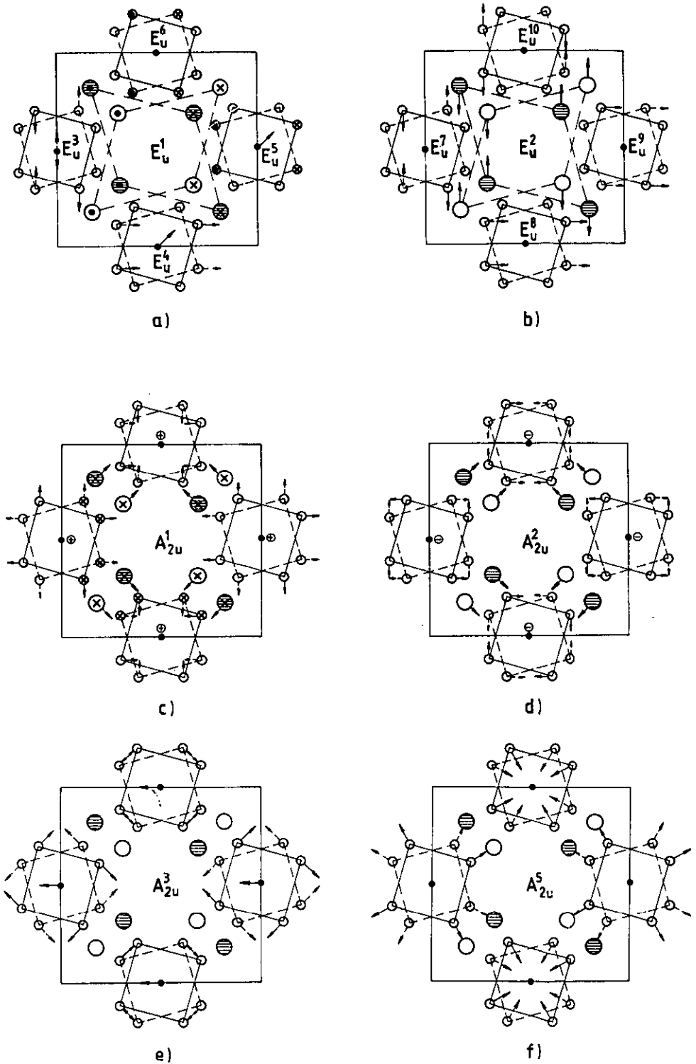
Figure 4. Normal-mode displacements of \text{Bi}_2\text{CuO}_4 for (a), (b) E_u and (c)-(f) A_{2u} infrared-active modes.
