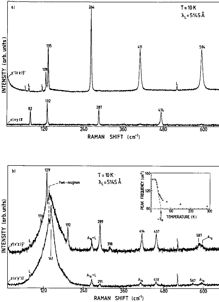
Figure 3. (a) Raman scattering spectra of \text{Bi}_2\text{CuO}_4 single crystals at 10 K for y'(z z) \bar{y}' and z(x y) \bar{z} polarizations; (b) the same spectra for y'(x' z) \bar{y}' and z(x' y') \bar{z} polarizations ( x \parallel [100] , y \parallel [010] , z \parallel [001] , x' \parallel [110] and y' \parallel [\bar{1}10] ).
